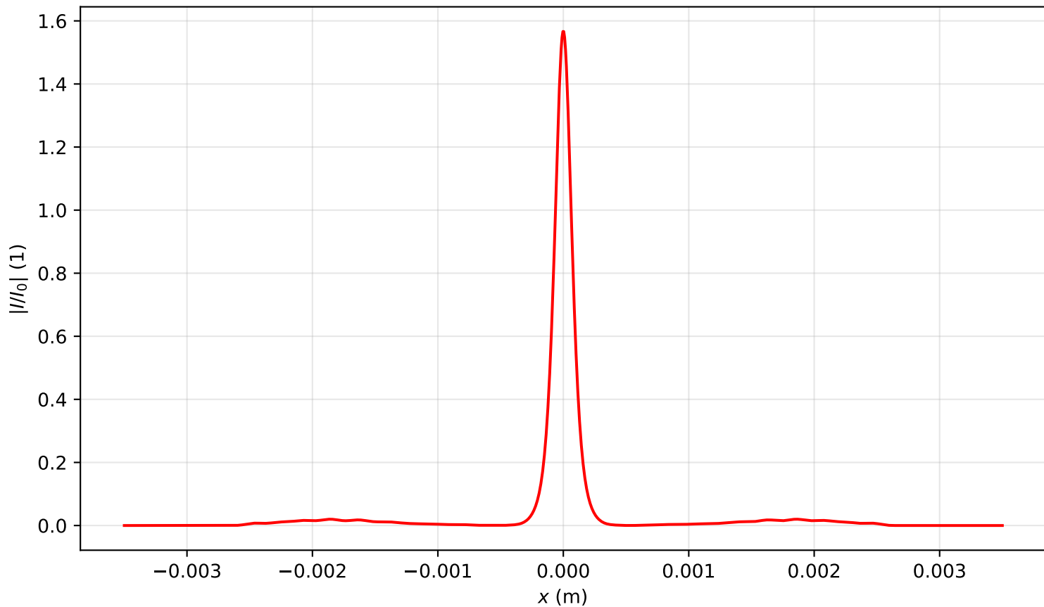
Intensity profile I(x, y = 0, z = 1.592)/I_0 , \text{Pin}=8.0\text{Pcr} , artificial time
